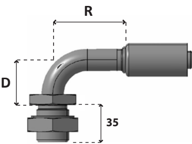
Bulkhead male insert O-ring, , 90° elbow
