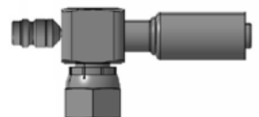
Short drop O-ring swivel - 90° block type - R134a valve - forward
