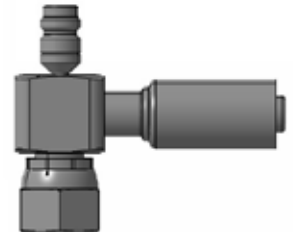
Short drop O-ring swivel - 90° block type - R134a valve - top
