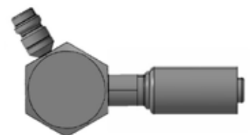
Tube-O HEX block 90° / R134a valve - 120°
