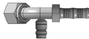
O-ring swivel R134a valve - right - 45°
