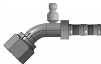
O-ring female swivel - switch adapter M10x1.25, 45° elbow
