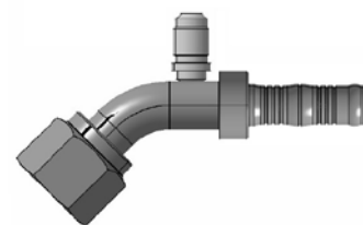
O-ring female swivel - pressure sensor 7/16-20 45° elbow
