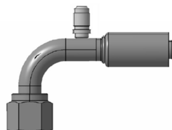
O-ring female swivel - pressure sensor 7/16-20 90° elbow
