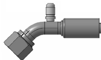
O-ring female swivel - pressure sensor 7/16-20 45° elbow
