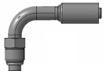
Short pilot O-ring male swivel, 90° elbow
