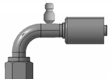
O-ring female swivel - switch adapter M10x1.25 90° elbow
