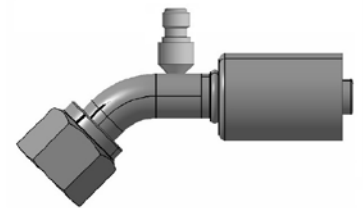
O-ring female swivel - switch adapter M10x1.25 45° elbow
