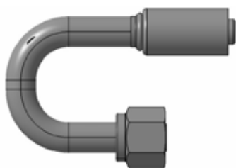
Long pilot O-ring swivel - tube connection, 180°
